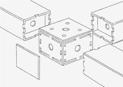
The extremely simple construction principle using the PIN connecting element means that the office system is highly flexible in terms of potential layouts.
