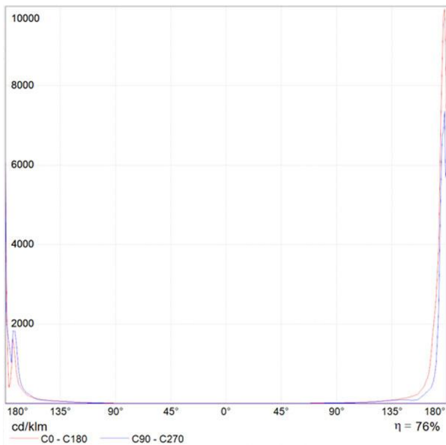
Cartesian diagram
