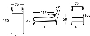
003.142.H.D BOOMERANG CHILL CHAISE BRAZO DCHO
