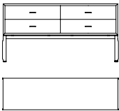
60001 Cassettiera a 4 cassetti in noce canaletto frontale cassetti in sycomore frisè tinto bianco Cabinet with 4 drawers in walnut canaletto drawers front in white painted fiddleback sycamore cm 158 x 42,5 x h 79,5 in 62 1/4 x 16 3/4 x h 31 1/4
