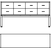
60007 Cassettiera a 8 cassetti in noce canaletto frontale cassetti con decorazione dorata in foglia Cabinet with 8 drawers in walnut canaletto drawers front with gold LEAF decoration cm 158 x 42,5 x h 79,5 in 62 1/4 x 16 3/4 x h 31 1/4
